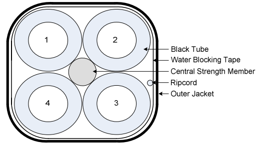
4-Tube Dielectric Low Shrink OSP Cable TC04MSOS
