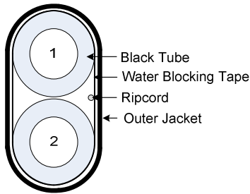
2-Tube Dielectric Low Shrink OSP Cable TC02MSOS
