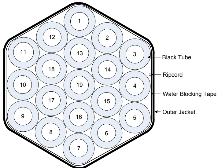
19-Tube Dielectric Low Shrink OSP Cable TC19MSOS
