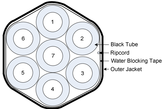
7-Tube Dielectric Low Shrink OSP Cable TC07MSOS
