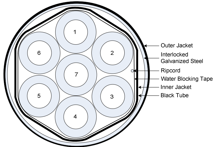
7-Tube Interlocked Armor / Dielectric OSP Cable TC07TOX-2
