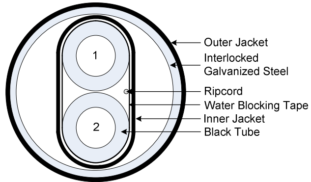
2-Tube Interlocked Armor / Dielectric OSP Cable TC02TOX-2
