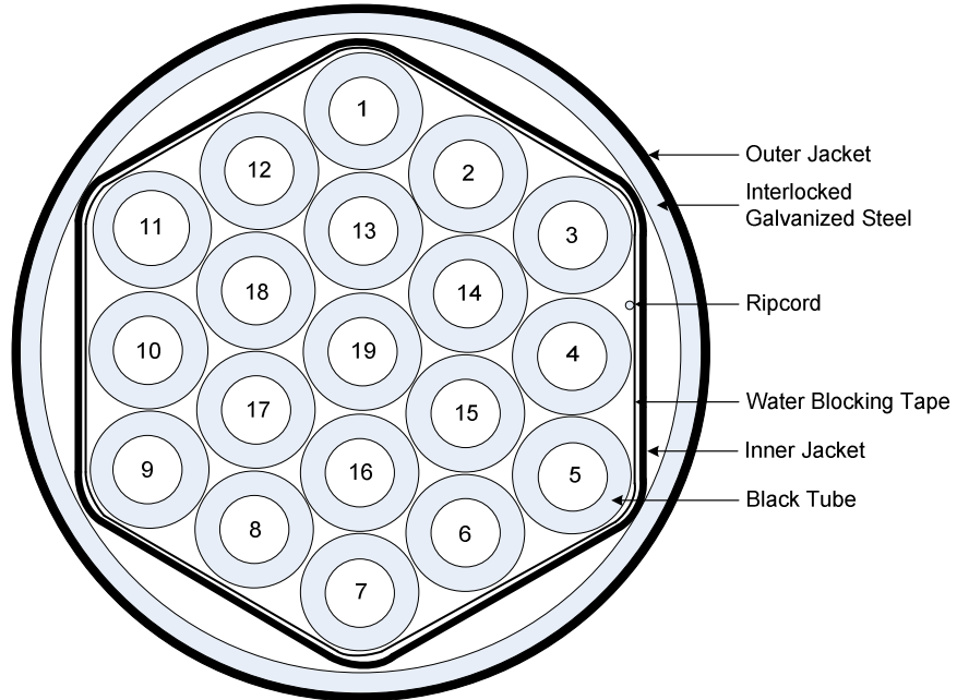
19-Tube Interlocked Armor / Dielectric OSP Cable TC19TOX-2
