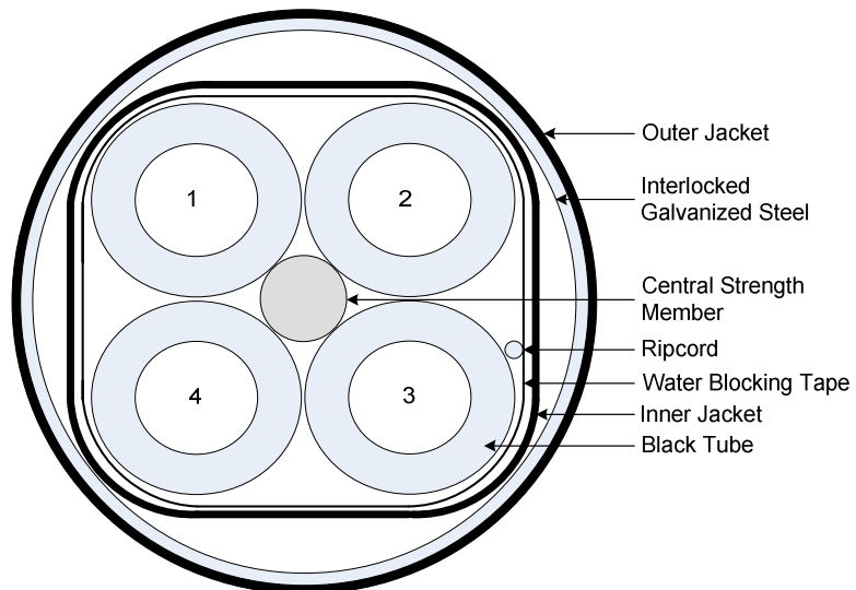
4-Tube Interlocked Armor / Dielectric OSP Cable TC04TOD-2
